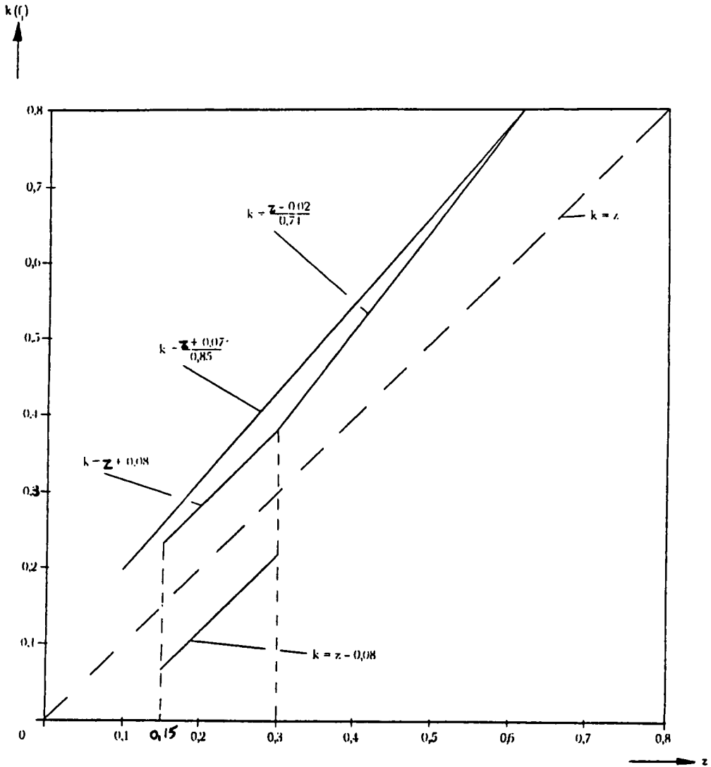
“Diagram 1 B. POWER-DRIVEN VEHICLES OTHER THAN THOSE OF CATEGORY M 1 “(See paragraph 3.1.1)
